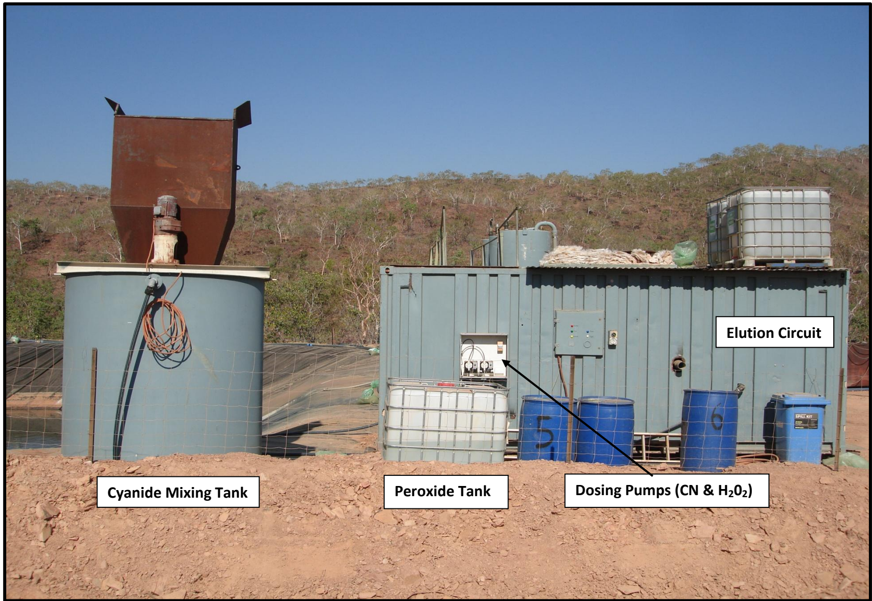
Our Vat Leach Setup
