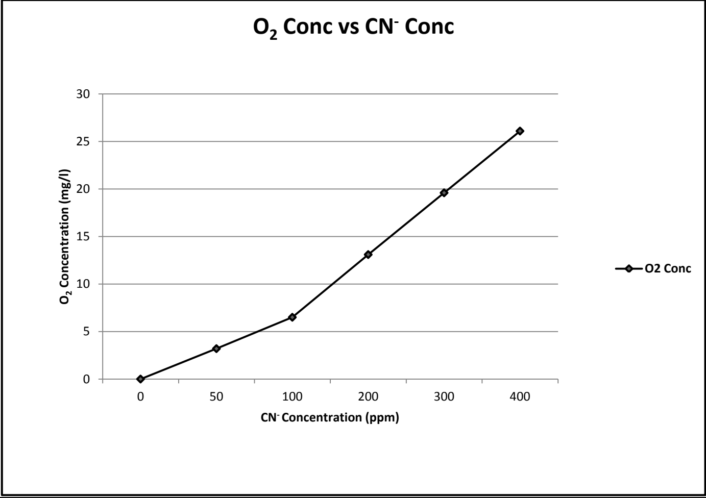
Graph of maximum oxygen concentration at varying cyanide levels
